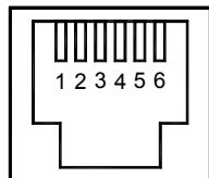
RS485 PORT - RJ11 (FROM RLC UNIT)
