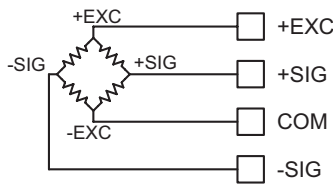
4-Wire Bridge Input
