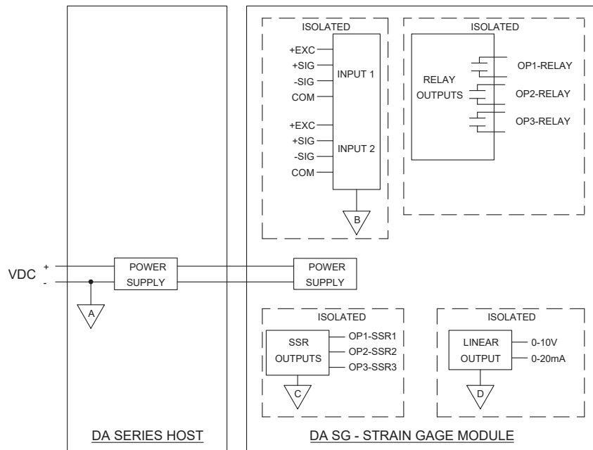
Block Diagram
