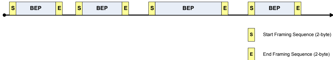
Figure 2: BEP Messages with Framing
