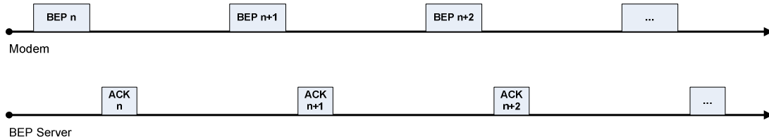
Figure 3: BEP Messages Acknowledgment
