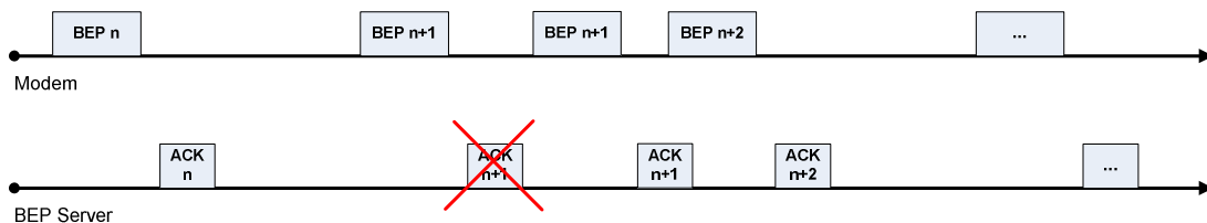
Figure 4: BEP Messages Acknowledgment with Retransmission
